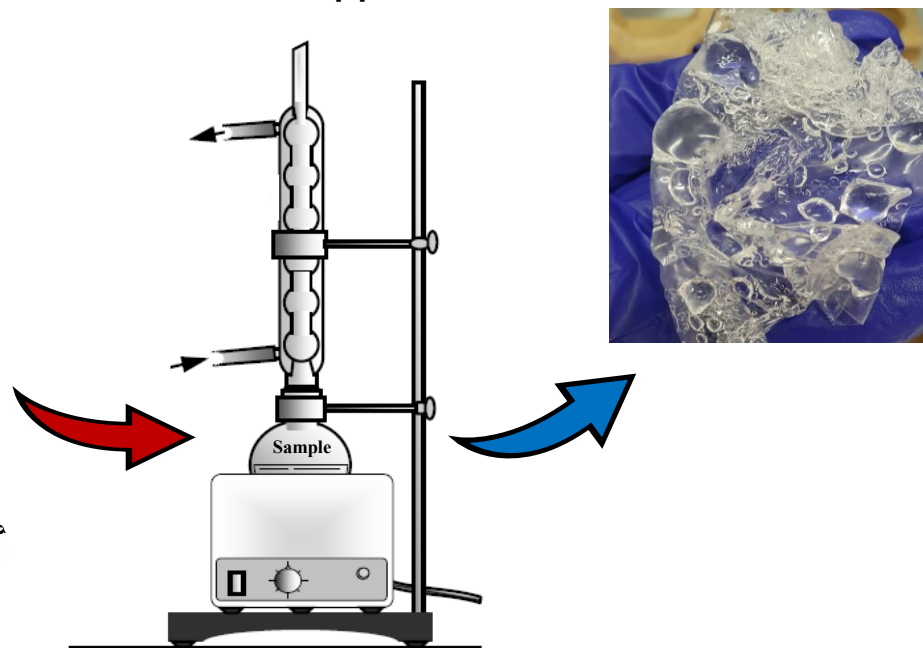
Extraction apparatus
